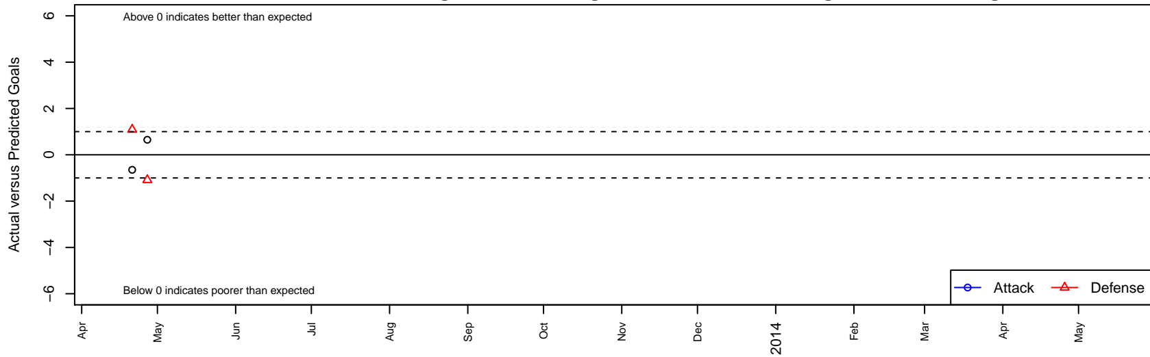
NEU Gamban B98 Dots are actual minus expected GF (blue circles) and GA (red triangles). Blue line is smoothed change in attack strength. Red is smoothed change in defense strength.
